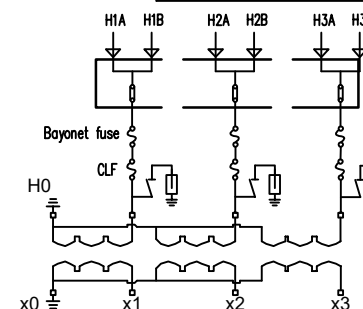
Wire Diagram
