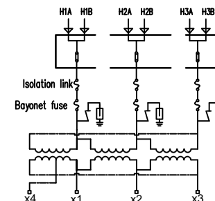
Wire Diagram
