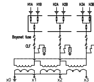
Wire Diagram
